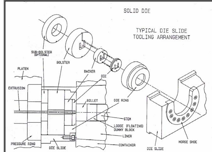
Flat (Solid) Die, no cavity or feeder, Tooling Arrangement
