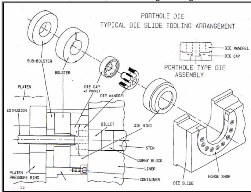
Hollow (Porthole) Die Tooling Arrangement
