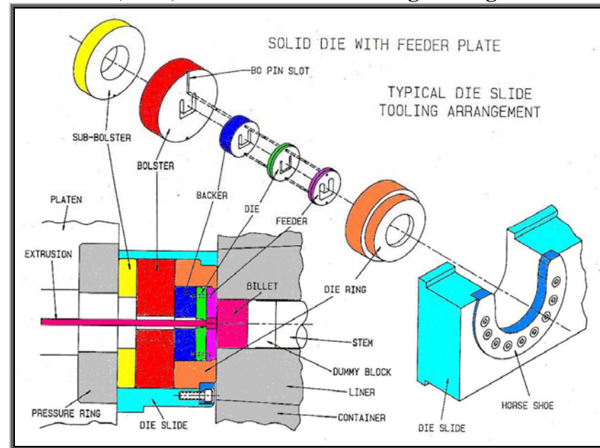
Flat (Solid) Die with Feeder Tooling Arrangement
