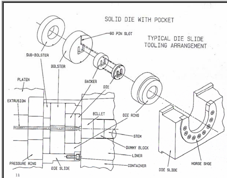
Flat (Solid) Die with Cavity Tooling Arrangement
